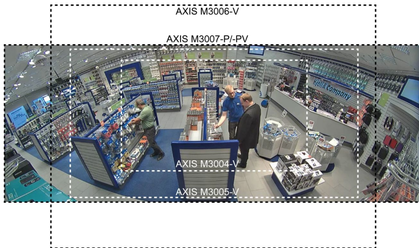
Left: Horizontal angles of view. Right: Approximate fields of view (AXIS M3007-P/-PV: wall-mount, panoramic view)
